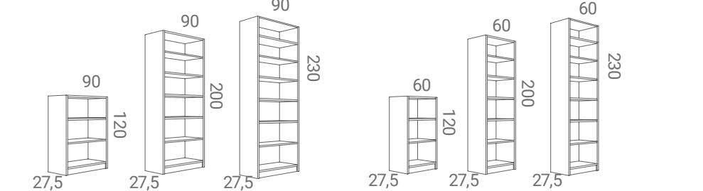
GRUNDSEKTION LG12090/LG20090/LG23090 GRUNDSEKTION LG12060/LG20060/LG23060
