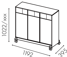
W7018 One-sided For 125 l bag
