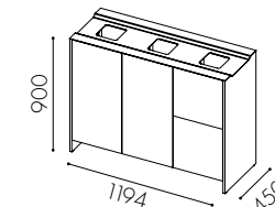
W99- 2 gaps for 2x125 l bag 2 drawers for 2x19 l bins
