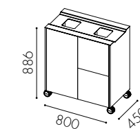
W97- 1 gap for 1x125 l bag 2 drawers for 2x19 l bins
