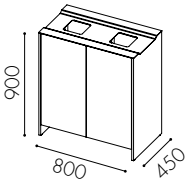
W91- 2 gaps for 2x125 l bag
