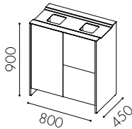
W98- 1 gap for 1x125 l bag 2 drawers for 2x19 l bins
