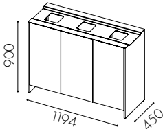
W92- 3 gaps for 3x125 l bag
