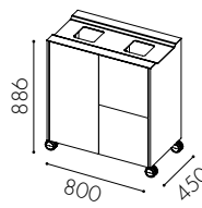
W97- 1 gap for 1x125 l bag 2 drawers for 2x19 l bins
