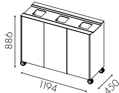
W94- 3 gaps for 3x125 l bag
