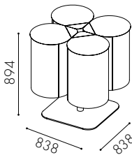
W8042 Covered lid W8043 Open lid Stand measurement: 600x600
