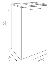
10 19 000- 190/l modul 750 x 650
